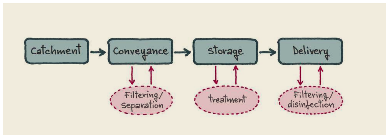
FIGURE 2.5.4 RAINWATER HARVESTING: PROCESS DIAGRAM FOR DRINKING WATER
