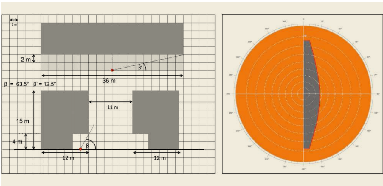
FIGURE A4.14 ARCADE FRONT VIEW AND SECTION (LEFT); OBSTRUCTION PROFILE FROM THE SELECTED POINT (RIGHT).
