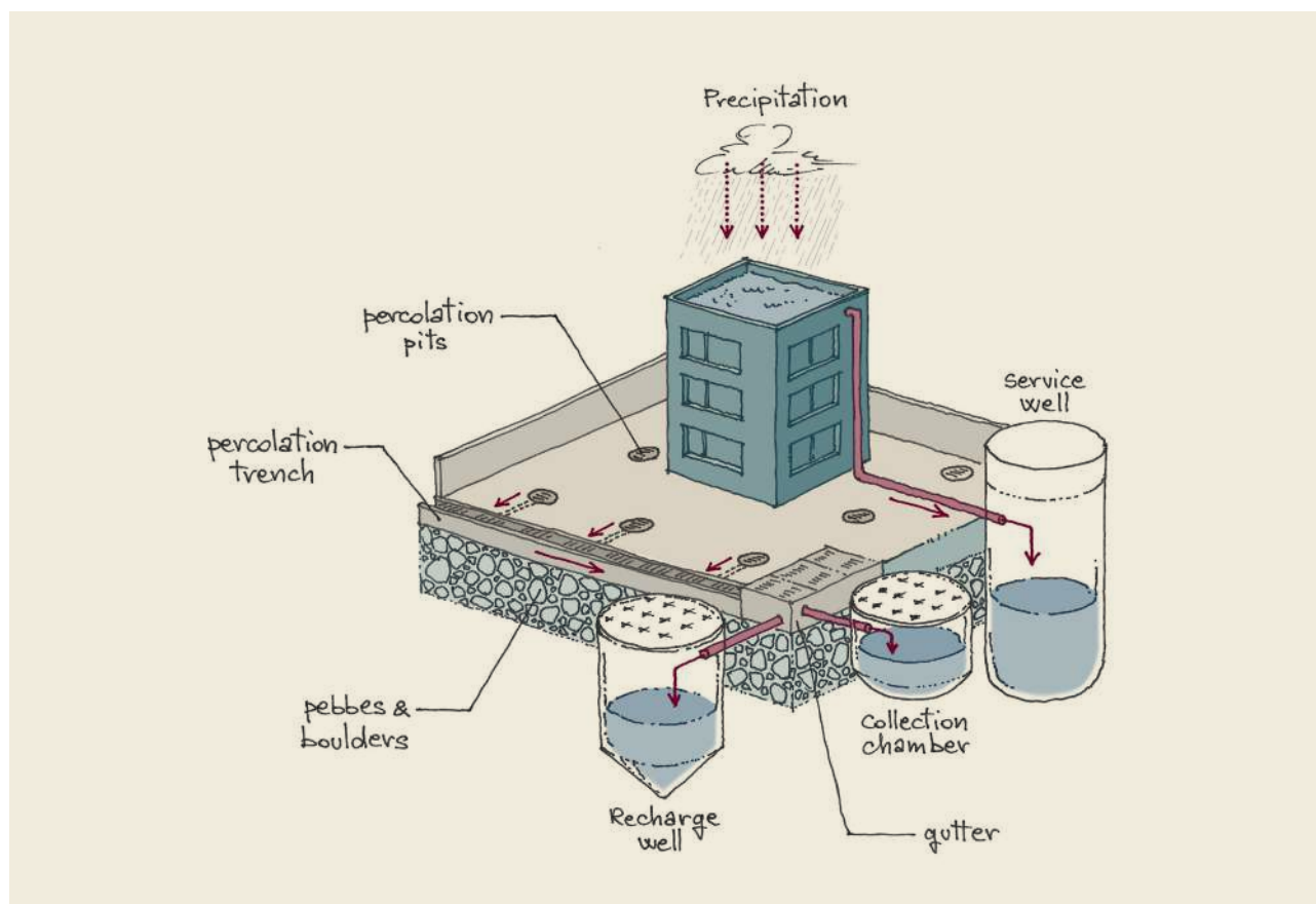
FIGURE 2.5.4 RAINWATER HARVESTING: PROCESS DIAGRAM FOR DRINKING WATER
