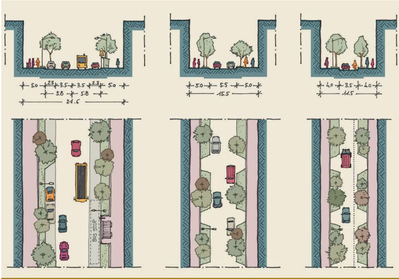
FIGURE 3.19 SHADOWED WALKWAYS
