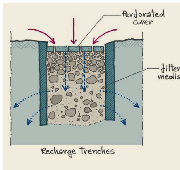
FIGURE 2.5.16 SECTION OF A RECHARGE TRENCH
