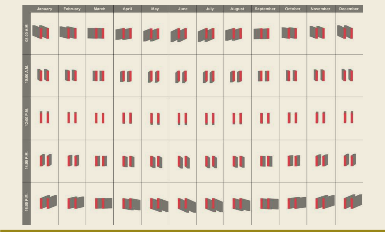
FIGURE 2.1.22 SUNSHINE AND SHADOW HOURS AT A POINT AT GROUND LEVEL, IN THE MIDDLE OF THE NORTH-SOUTH CANYON SKETCHED IN FIGURE A3.4, AT 7S LATITUDE
