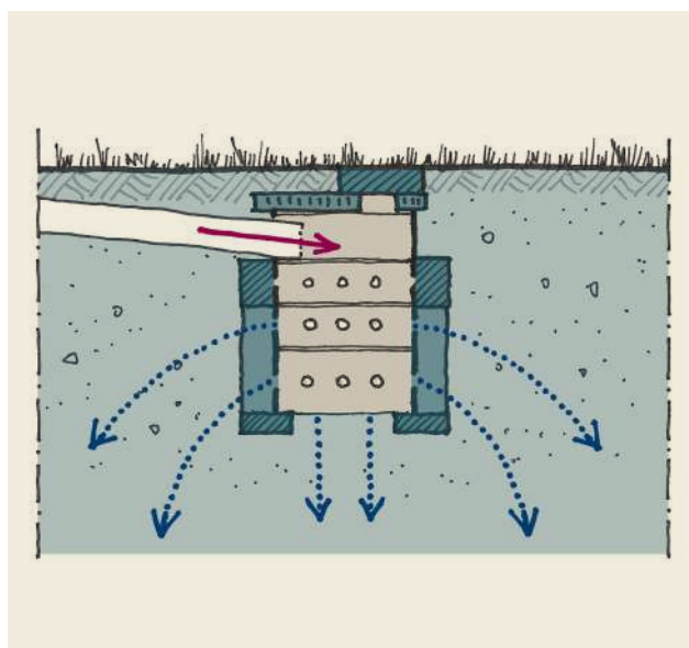
FIGURE 2.5.15 SKETCH OF A RECHARGE PIT
