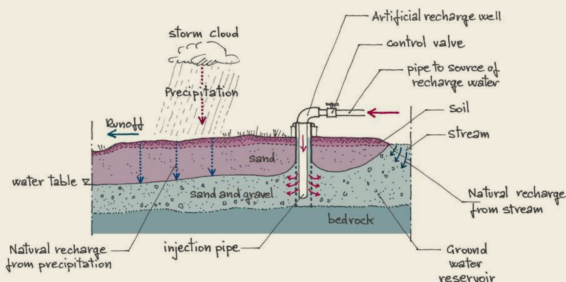
FIGURE 2.5.23 ARTIFICIAL RECHARGE OF GROUNDWATER (USGS 2016)
