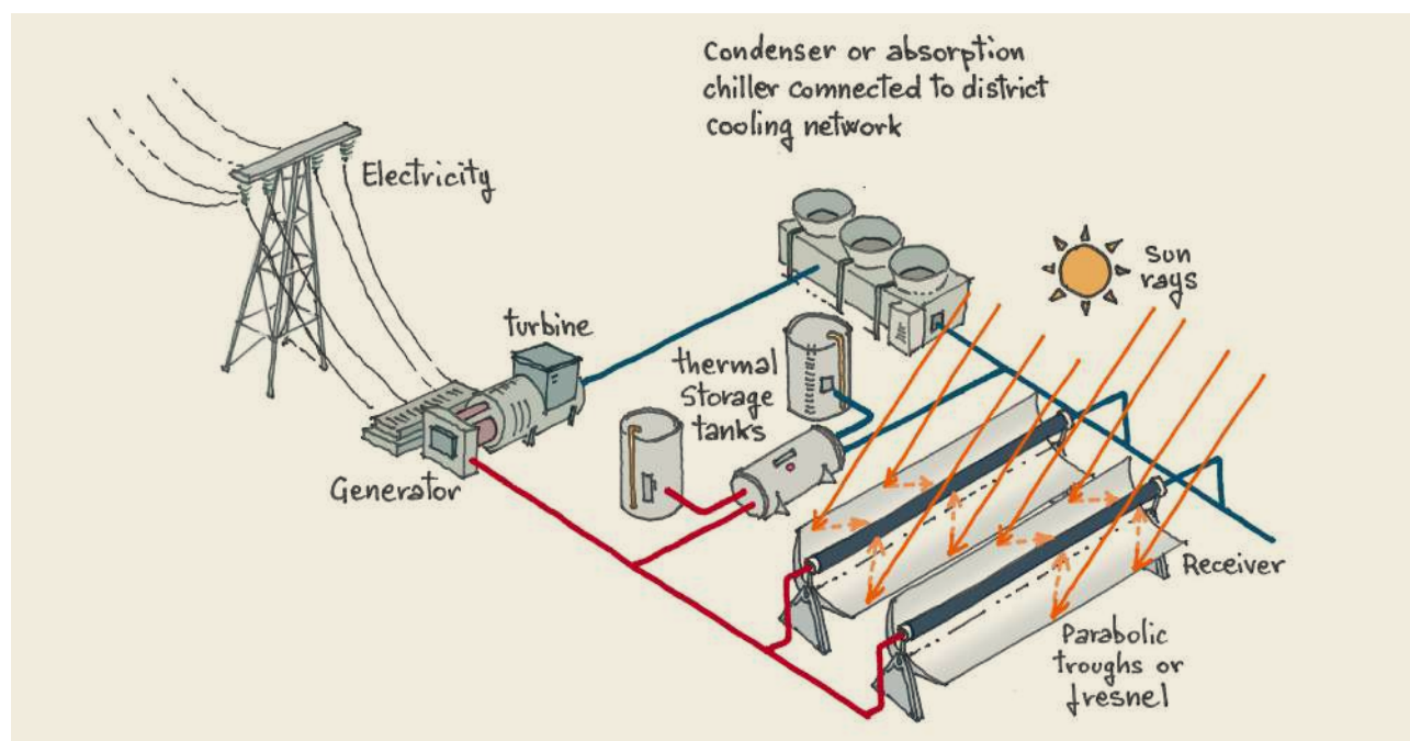
FIGURE A5.6 PARABOLIC THROUGH SOLAR POWER PLANT
