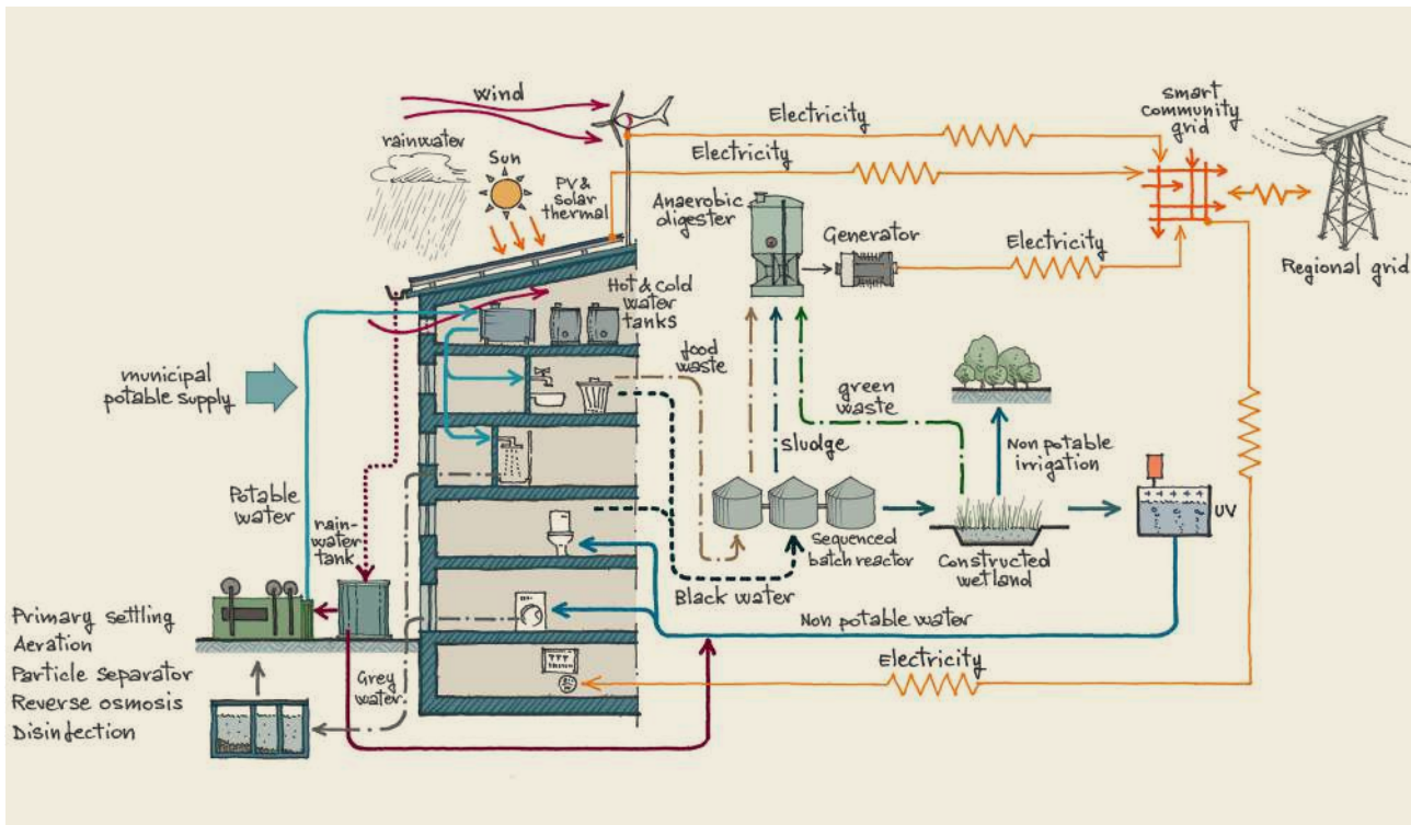
FIGURE 2.7.2 SCHEMATIC OF INTEGRATED WATER, WASTE AND ENERGY SYSTEMS FOR A SUSTAINABLE NEIGHBOURHOOD. ADAPTED FROM THE QUINDAO ECOBLOCK (SEE CHAPTER 4 FOR MORE INFORMATION))
