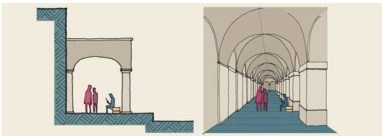
FIGURE 2.1.25 ARCADES
