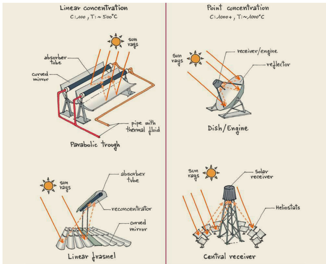
FIGURE A5.6 PARABOLIC THROUGH SOLAR POWER PLANT
