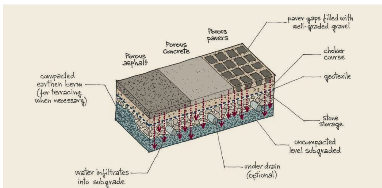
FIGURE 2.1.41 TYPES OF POROUS PAVEMENTS
