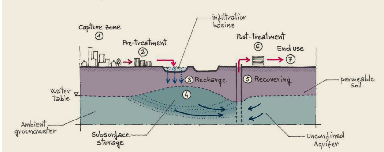
FIGURE 2.5.22 SCHEMATIC OF THE TREATED WASTEWATER AQUIFER RECHARGE PROCESS (ADAPTED FROM: SSWM 2017)
