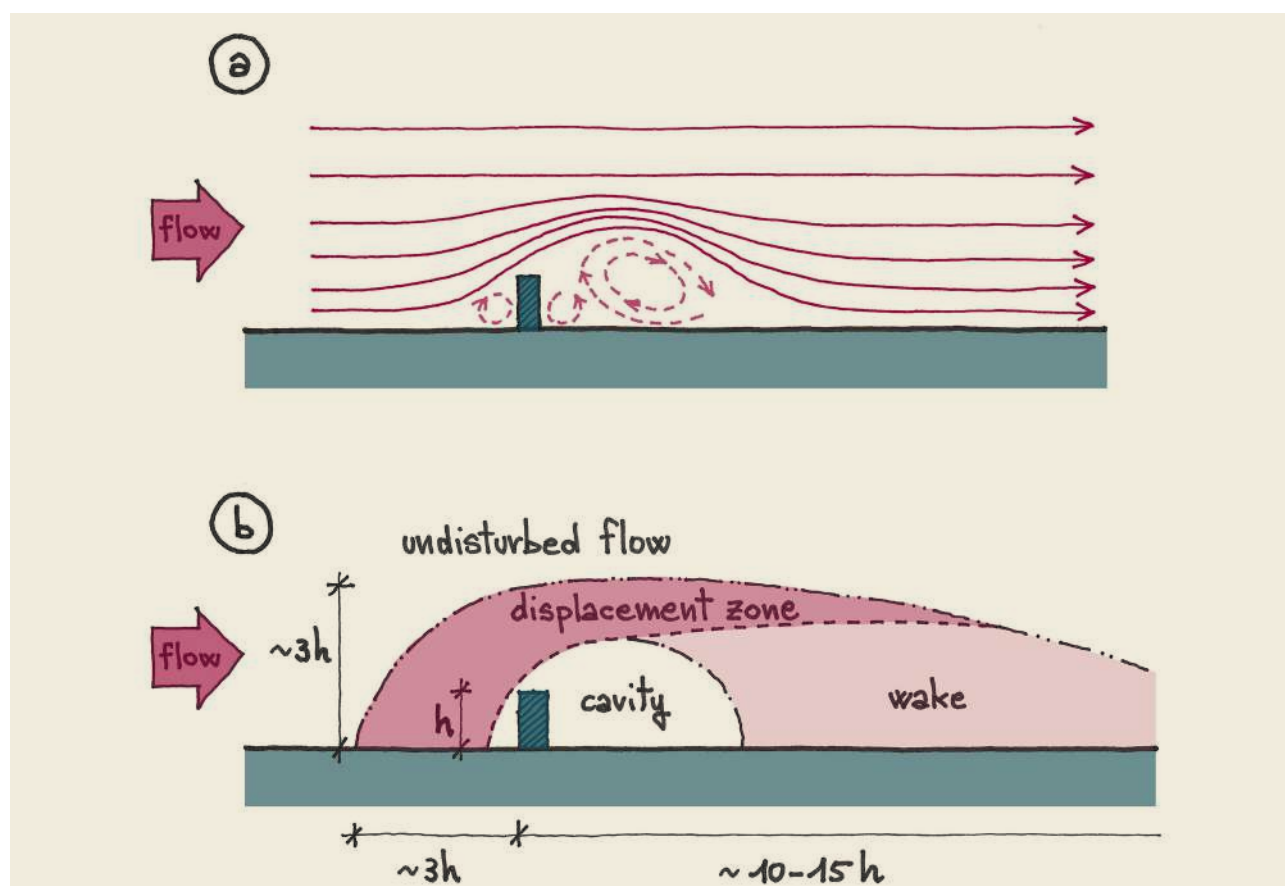
FIGURE A1.24 (A) STREAMLINES AND (B) GENERALISED ZONES ASSOCIATED WITH THE TYPICAL PATTERN OF AIRFLOW INDUCED BY A SOLID BARRIER PLACED NORMAL TO THE FLOW. DIMENSIONS EXPRESSED AS MULTIPLES OF THE BARRIER HEIGHT, h (ADAPTED FROM: OKE 1978).
