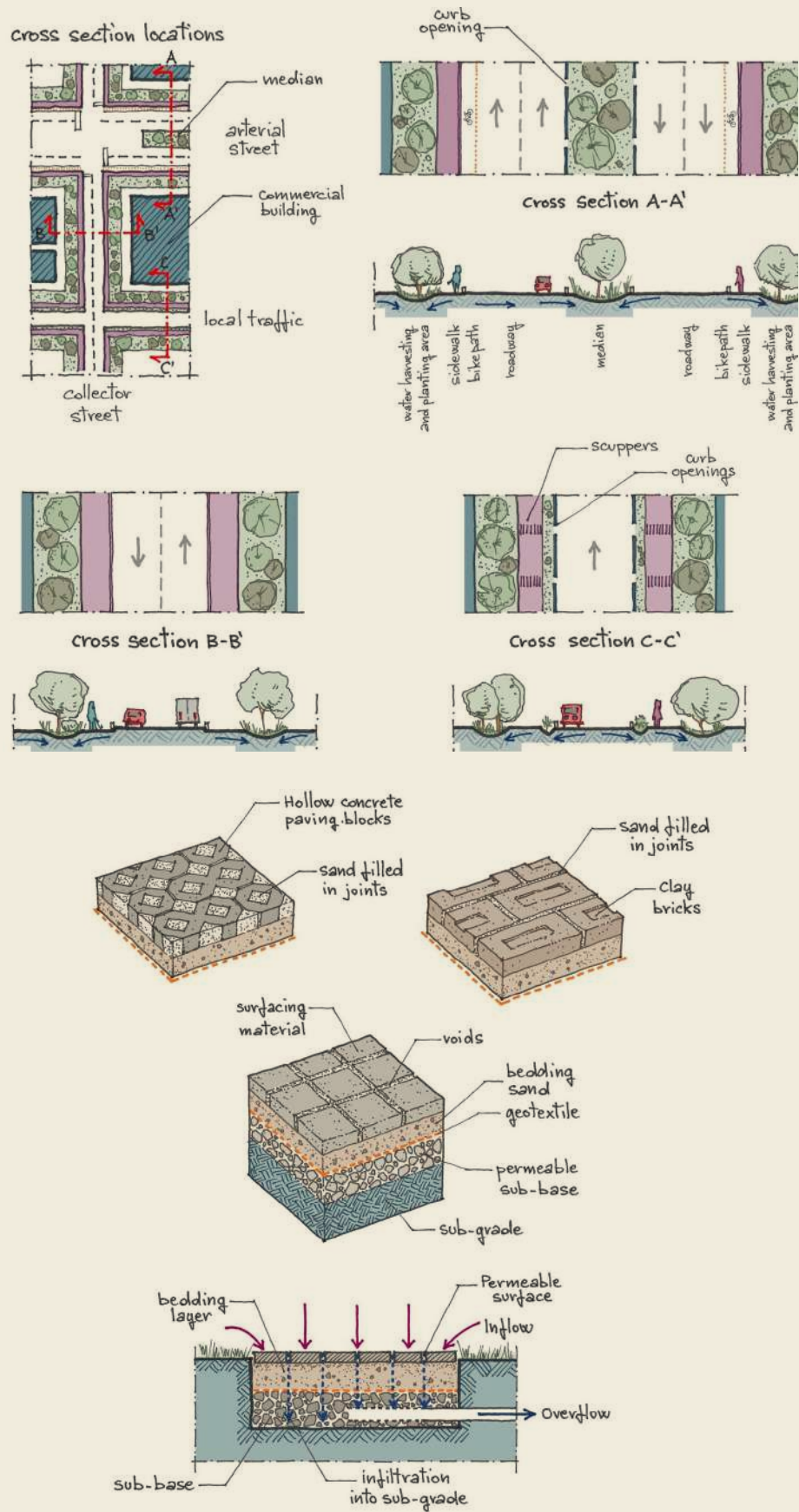
FIGURE 3.23 MAXIMISE PERVIOUS SURFACES
