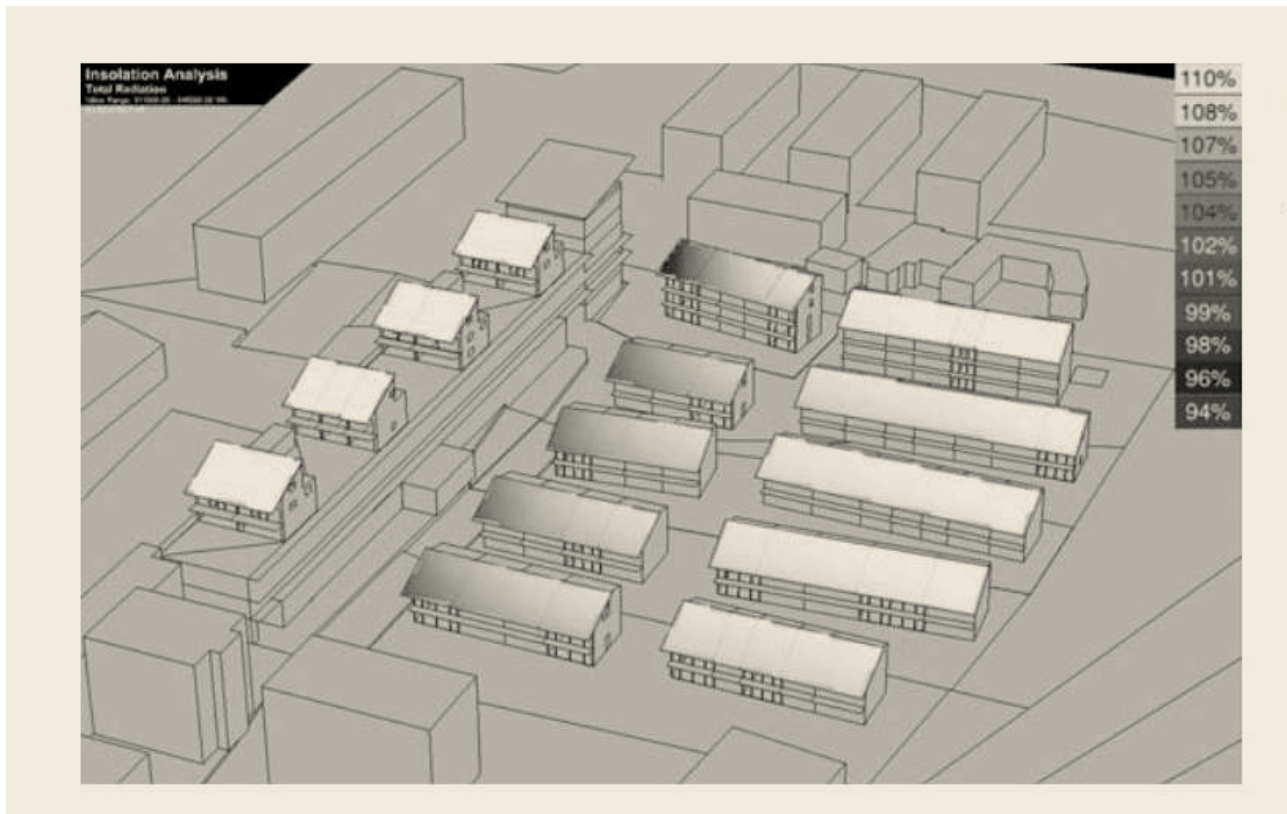
FIGURE 4.33 SOLAR POTENTIAL (SOURCE: HEINZE 2009)
