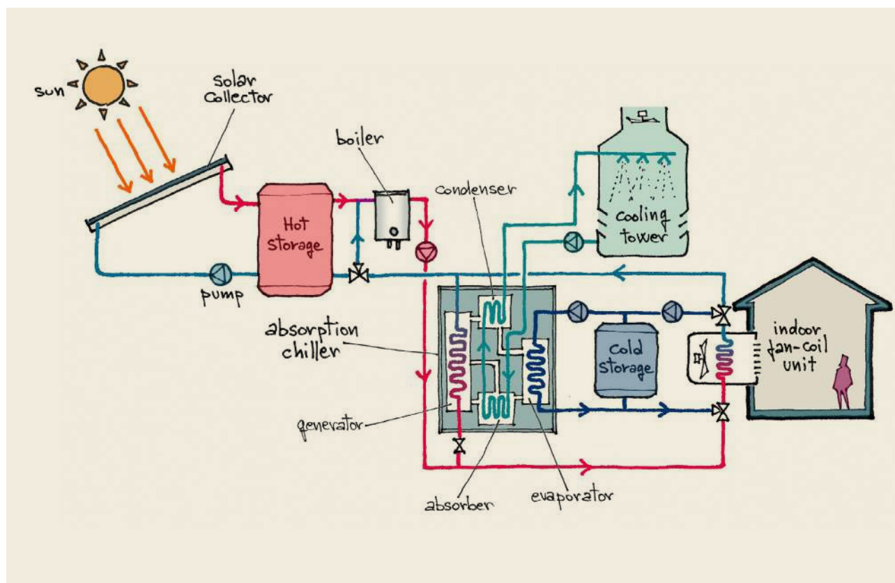
FIGURE A5.3 SOLAR POWERED AIR CONDITIONING SYSTEM
